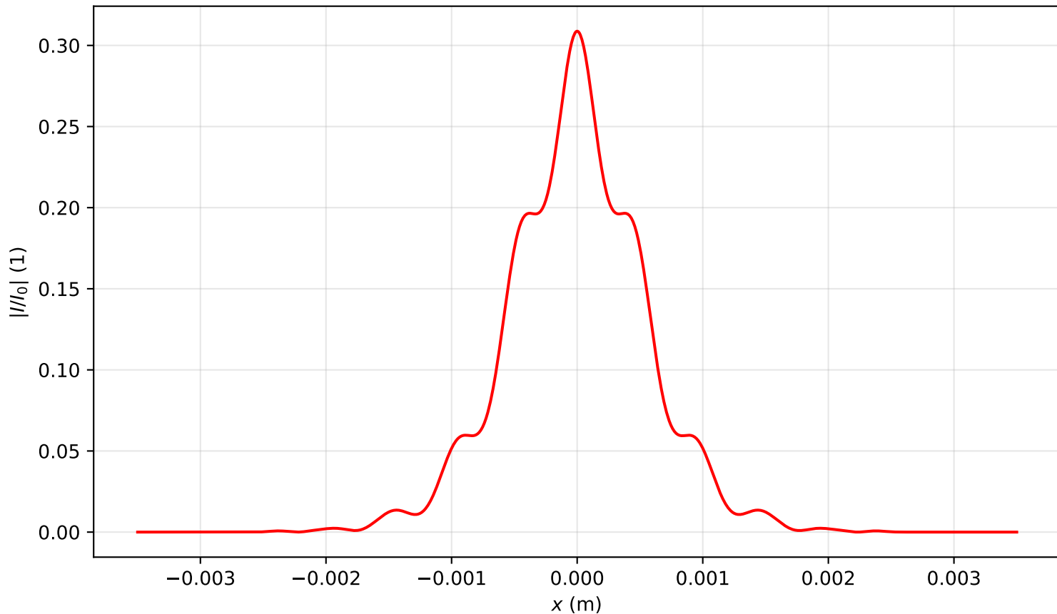
Intensity profile I(x, y = 0, z = 3.344)/I_0 , P_{in}=1.0P_{cr} , artificial time
